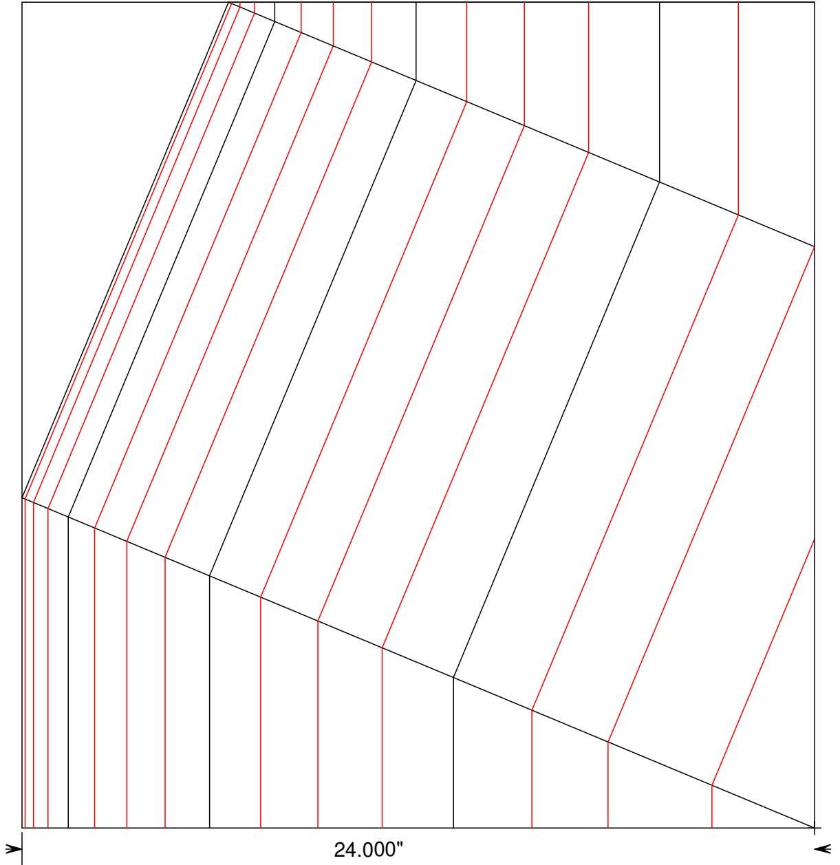
Chine And Sheer Body View for Fig 3.6A
